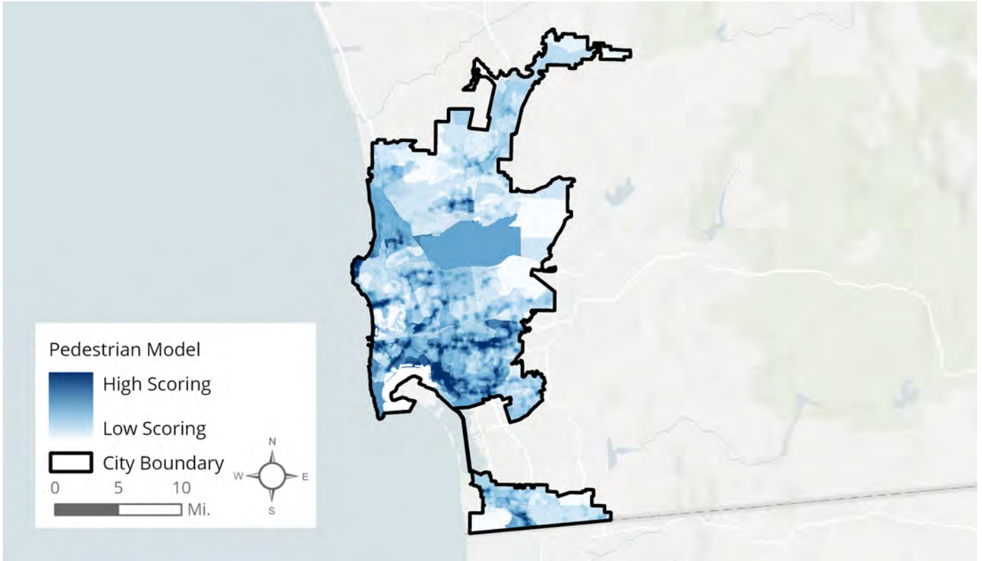
FIGURE 6-2: Pedestrian Model
