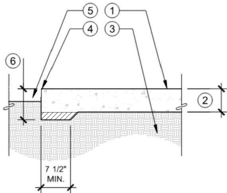
A WALKWAY DETAIL NOT TO SCALE
