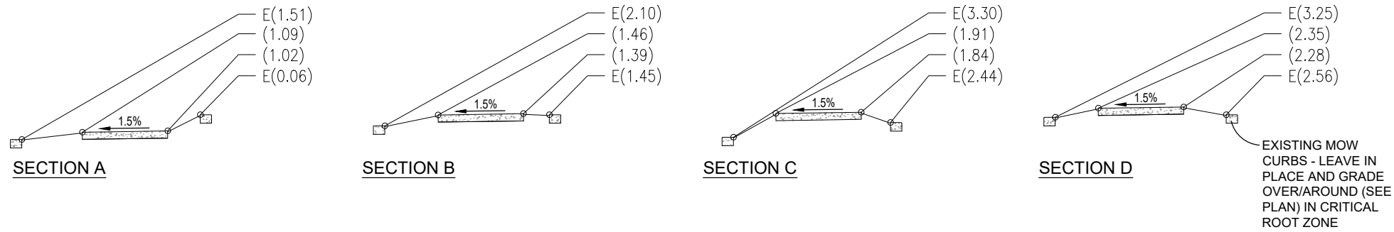
B WALKWAY SECTIONS SCALE: 1/8" = 1'-0"
