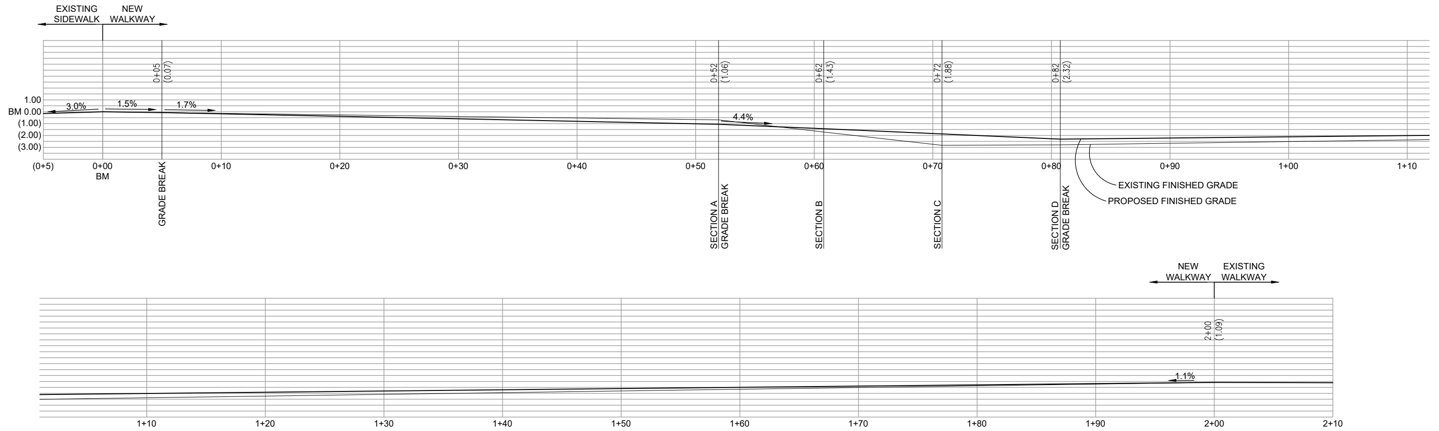
A WALKWAY PROFILE SCALE: 1/8" = 1'-0"
