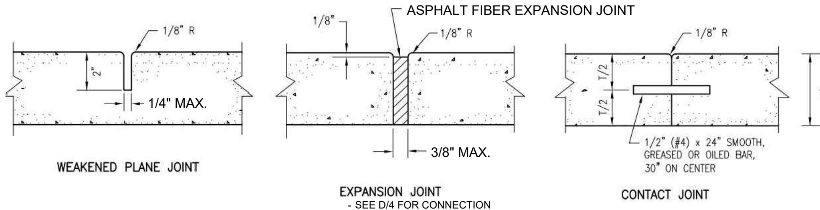
B CONSTRUCTION JOINTS NOT TO SCALE
