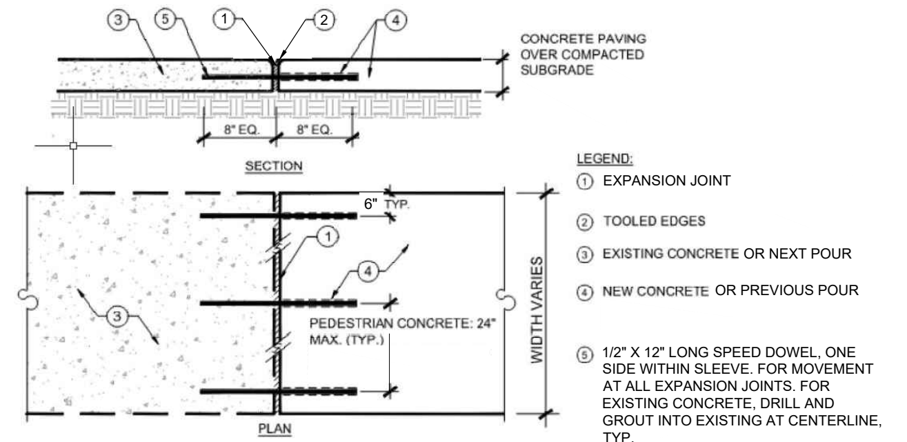
D CONCRETE PAVING CONNECTION NOT TO SCALE
