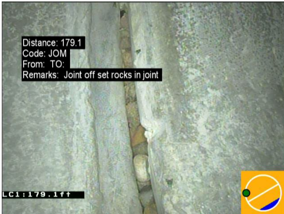
CCTV of offset joint within 30-Inch RCP
