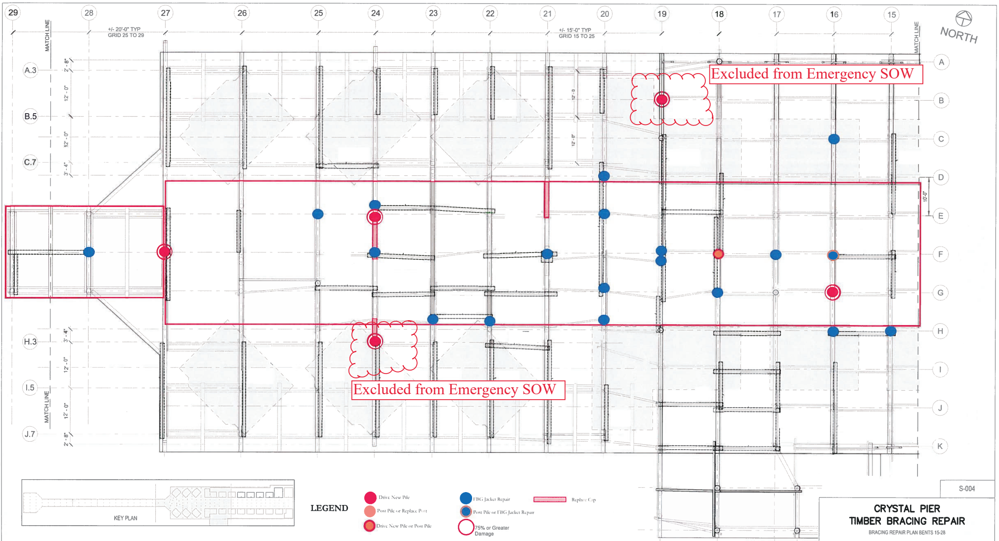
PIER FRAMING PLAN - BENTS 15-28 SCALE 1/8"=1'-0"
