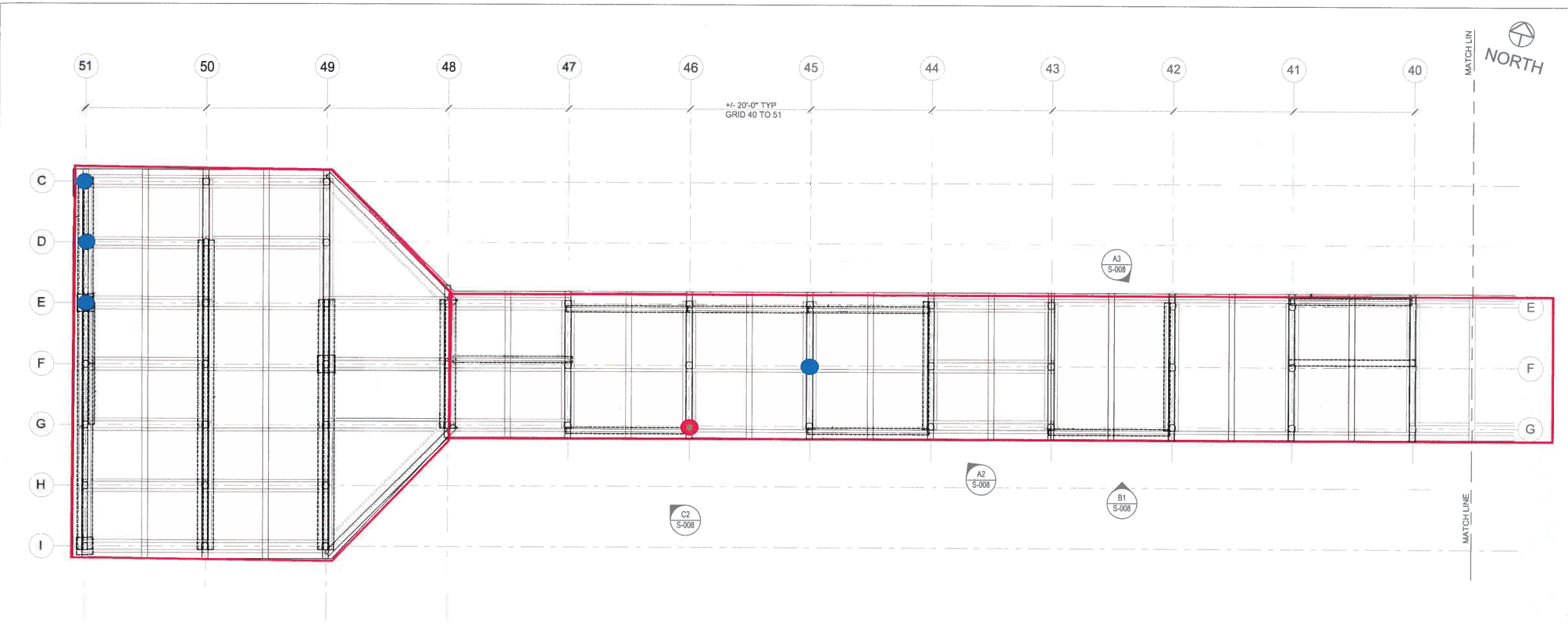
PIER FRAMING PLAN - BENTS 40-51 SCALE: 1/8"=1'-0"
