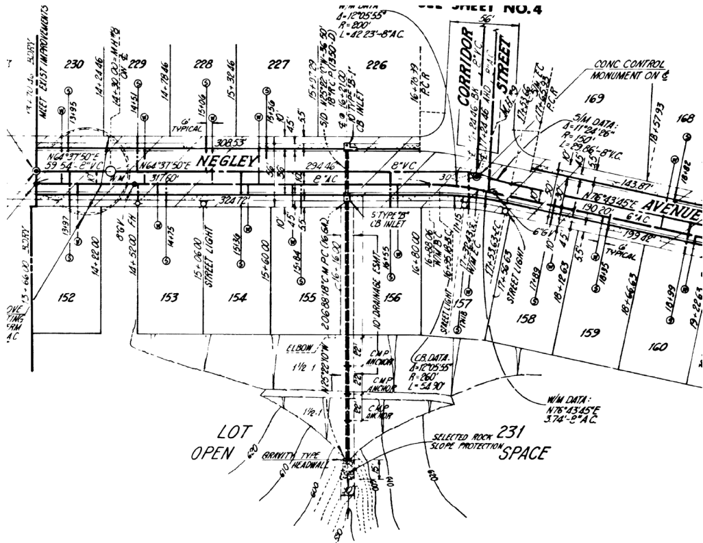
Plan View - Drawing # 14075-5-D
