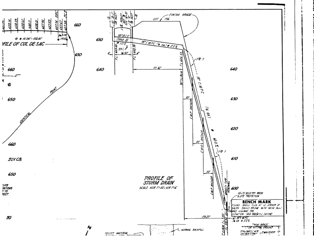
Profile View - Drawing # 14075-5-D
