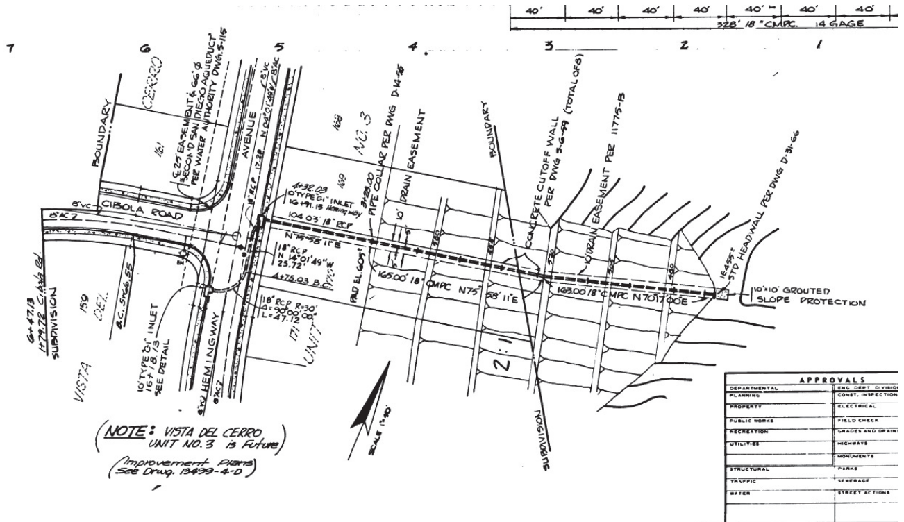
Plan View – Drawing # 13499-5-D
