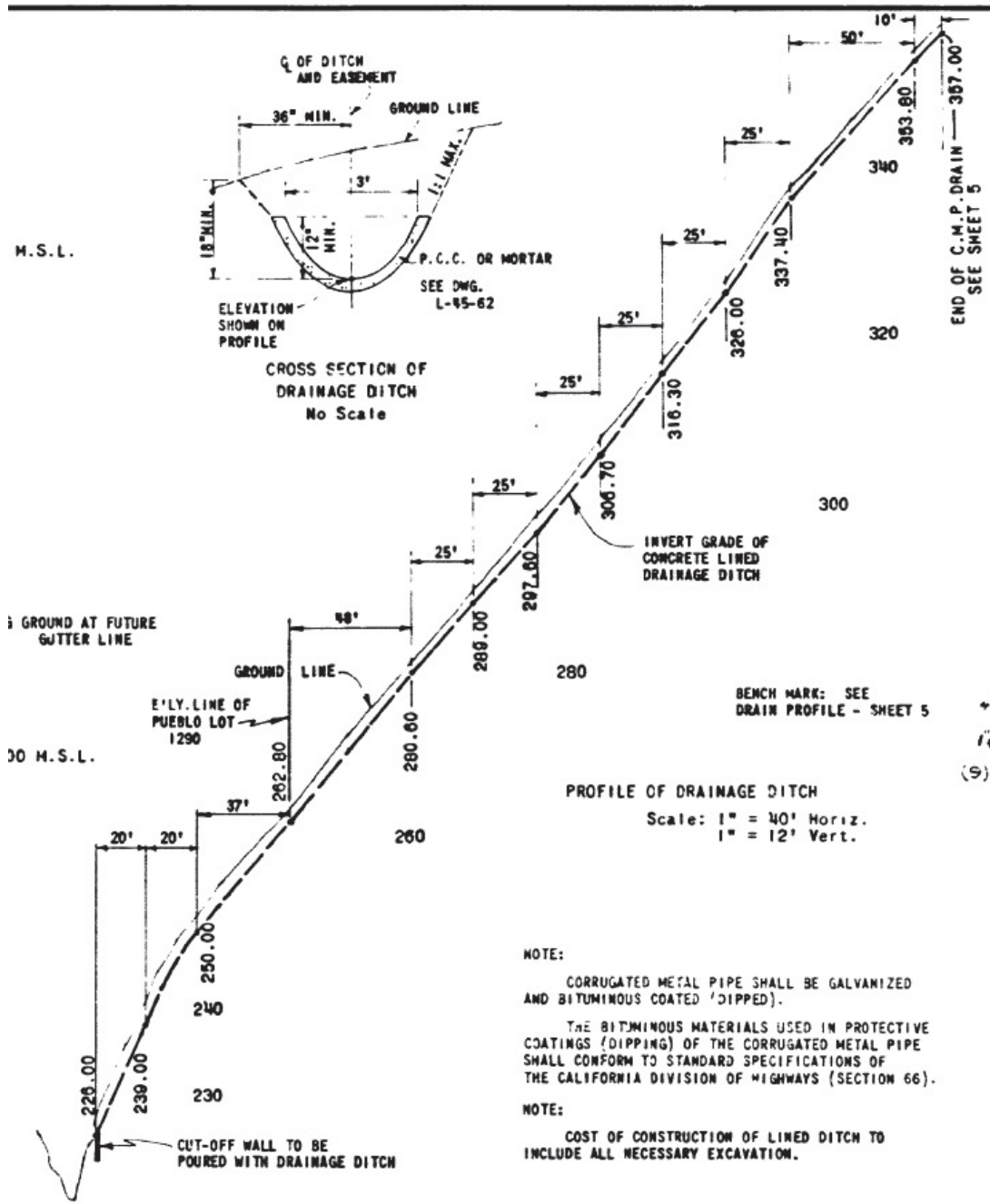
Profile - Drawing # 11495-1-D
