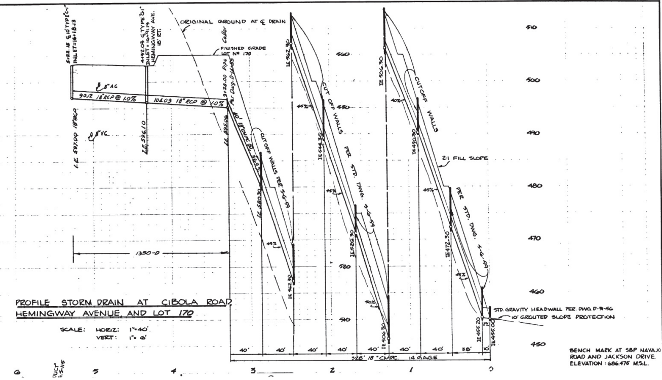
Profile View – Drawing # 11495-5-D
