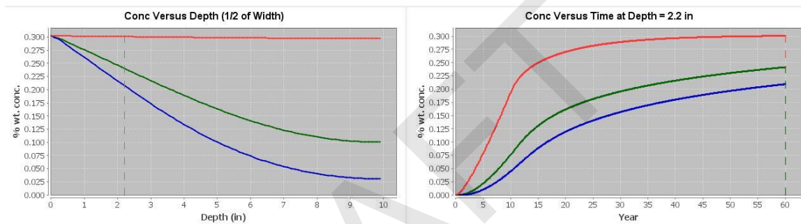
Figure 11 TI sample 11/ MN Sample 7N- Pile Top North Side
