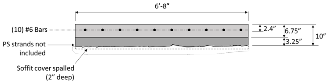
FIGURE 4: Midspan Section – Damaged Condition
