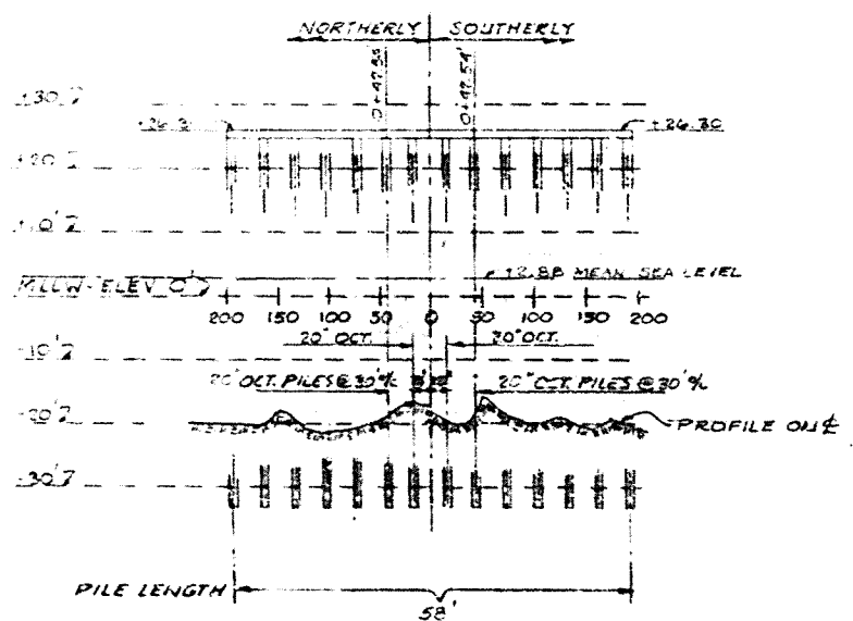
PROFILE ON \phi OF PIER AT END INTERSECTION
