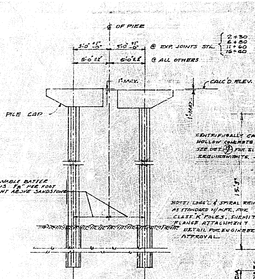
PIER SECTION SHOWING PLACING TOLERANCES SCALE: 1/4" = 1'-0"
