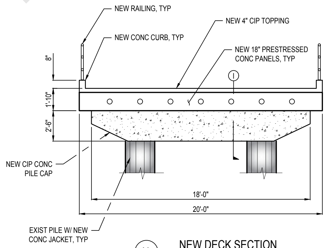
I NEW DECK SECTION NO SCALE
