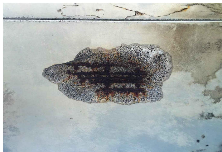
UNDERDECK DAMAGE
