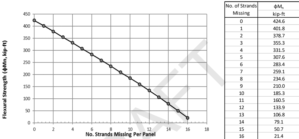
FIGURE 5: Midspan Section – Positive Moment Strength Corresponding to Number of Strands Lost
