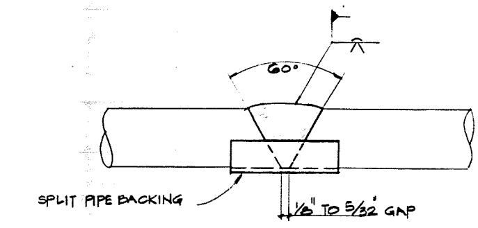
INDIRECT BUTT SPLICE
