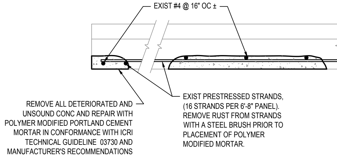
B2 SECTION NO SCALE
