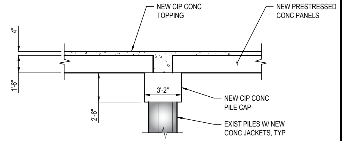
I NEW DECK SECTION NO SCALE
