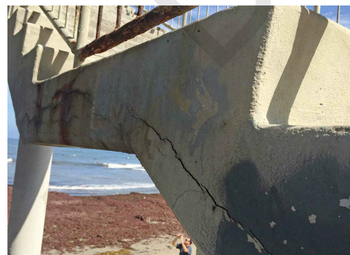
CONCRETE STAIR DAMAGE
