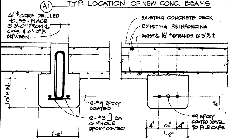
A1 TYP. LOCATION OF NEW CONC. BEAMS A2 NEW CONC. BMS. BETWEEN PILE CAPS
