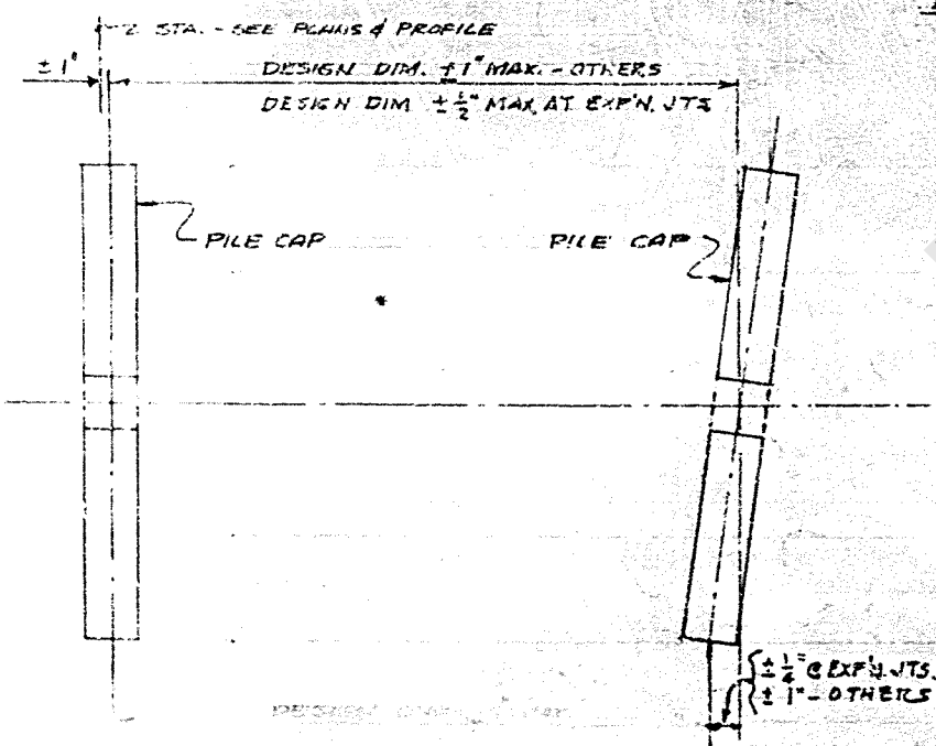
PIER PLAN SHOWING PLACING TOLERANCES SCALE: 1/4" = 1'-0"
