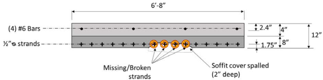
Figure 17 - Midspan Section of Precast Panel
