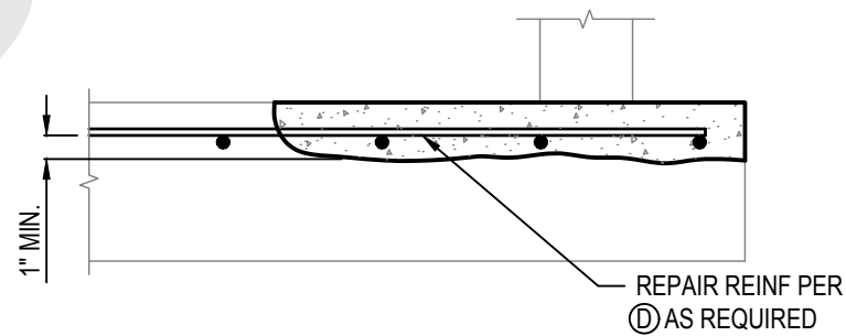
C3 SECTION NO SCALE
