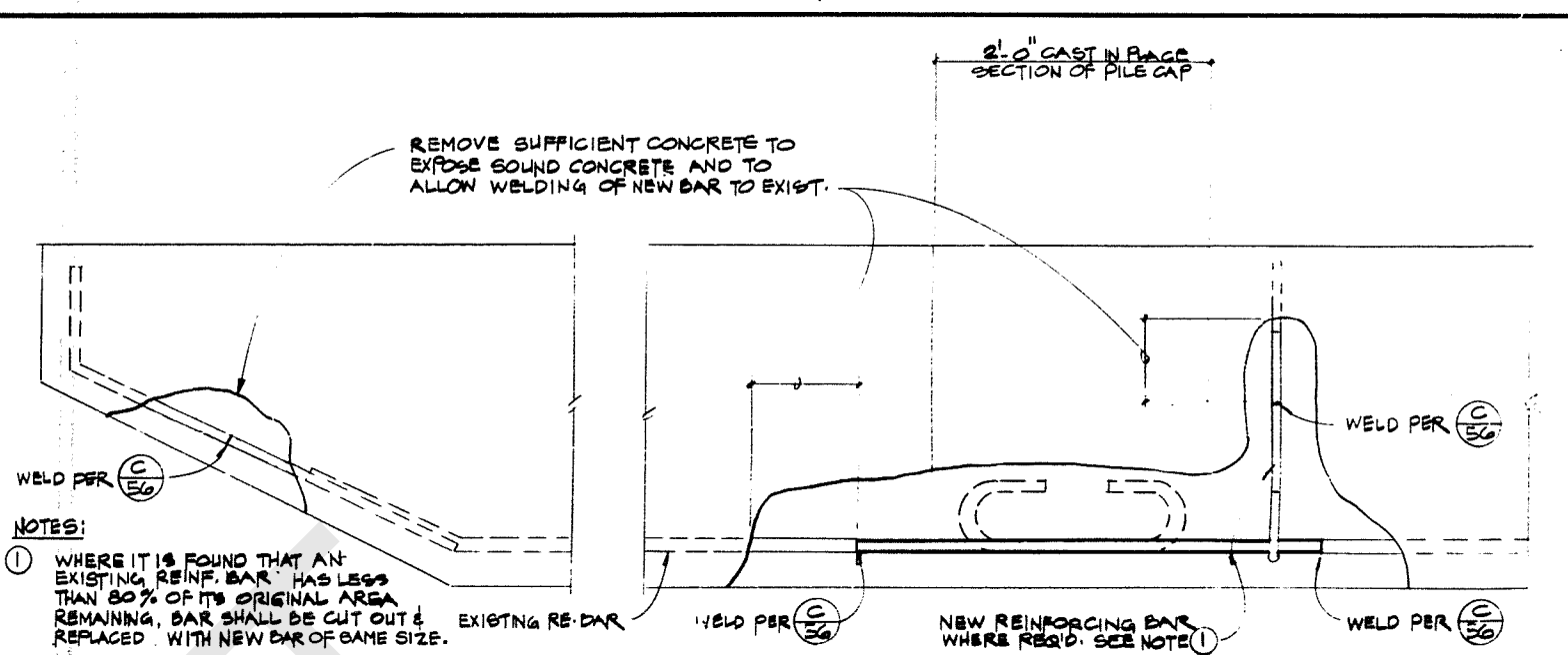
D 56 REPAIR FOR REINFORCING IN PILE CAPS
