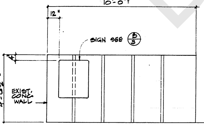
SIGN LOCATION 1/2" = 1'-0"
