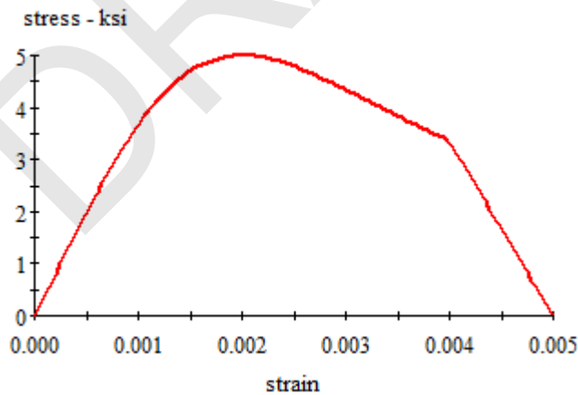
FIGURE 10: Nominal Unconfined Concrete Material Model (5ksi)
