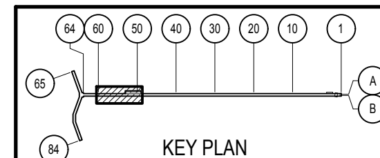
PARTIAL SOFFIT DECK PLAN - 5 SCALE: 1"=30'-0"
