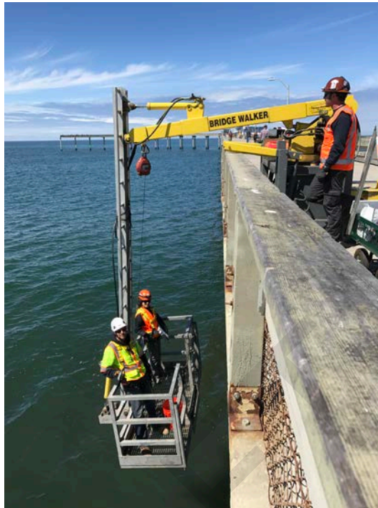
Figure 5 - Snooper used for under deck inspection
