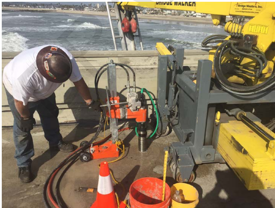
Figure 6 - Coring of the deck
