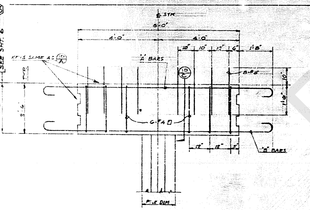
10 D SPECIAL PILE CAP DETAIL SCALE: 1/4" = 1'-0"
