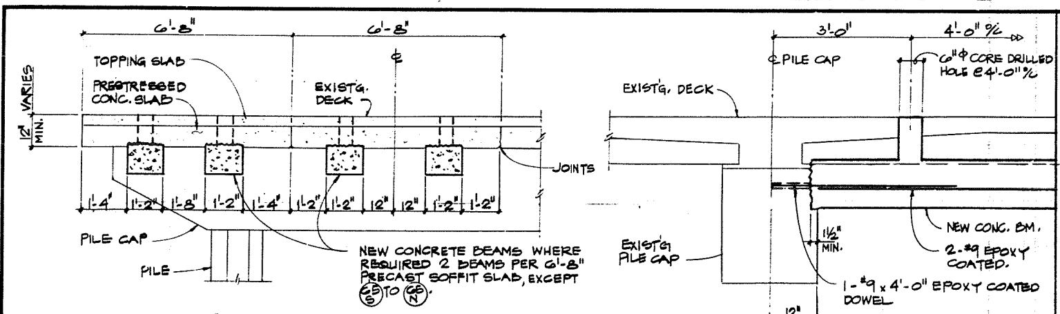
A3 CONN. OF NEW BM. TO EXIST. PILE CAPS
