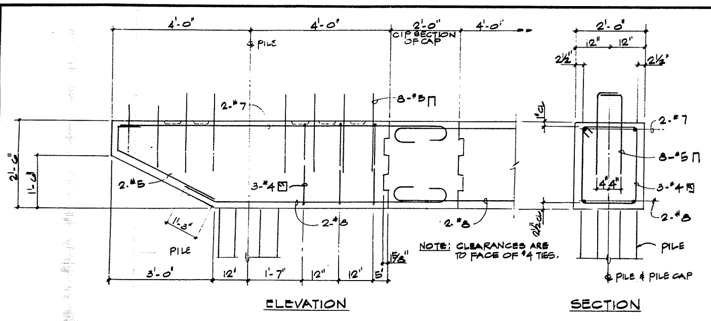
A 56 EXISTING PILE CAP - DIMENSIONS AND REINFORCING PER AS-BUILT DRAWINGS OF ORIGINAL PIER 3/4" = 1'-0"
