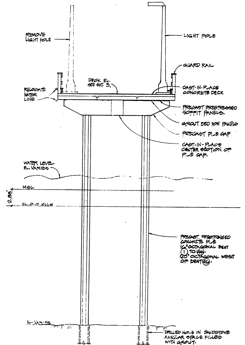
(A/2) PIER SECTION 1/4" = 1'-0"
