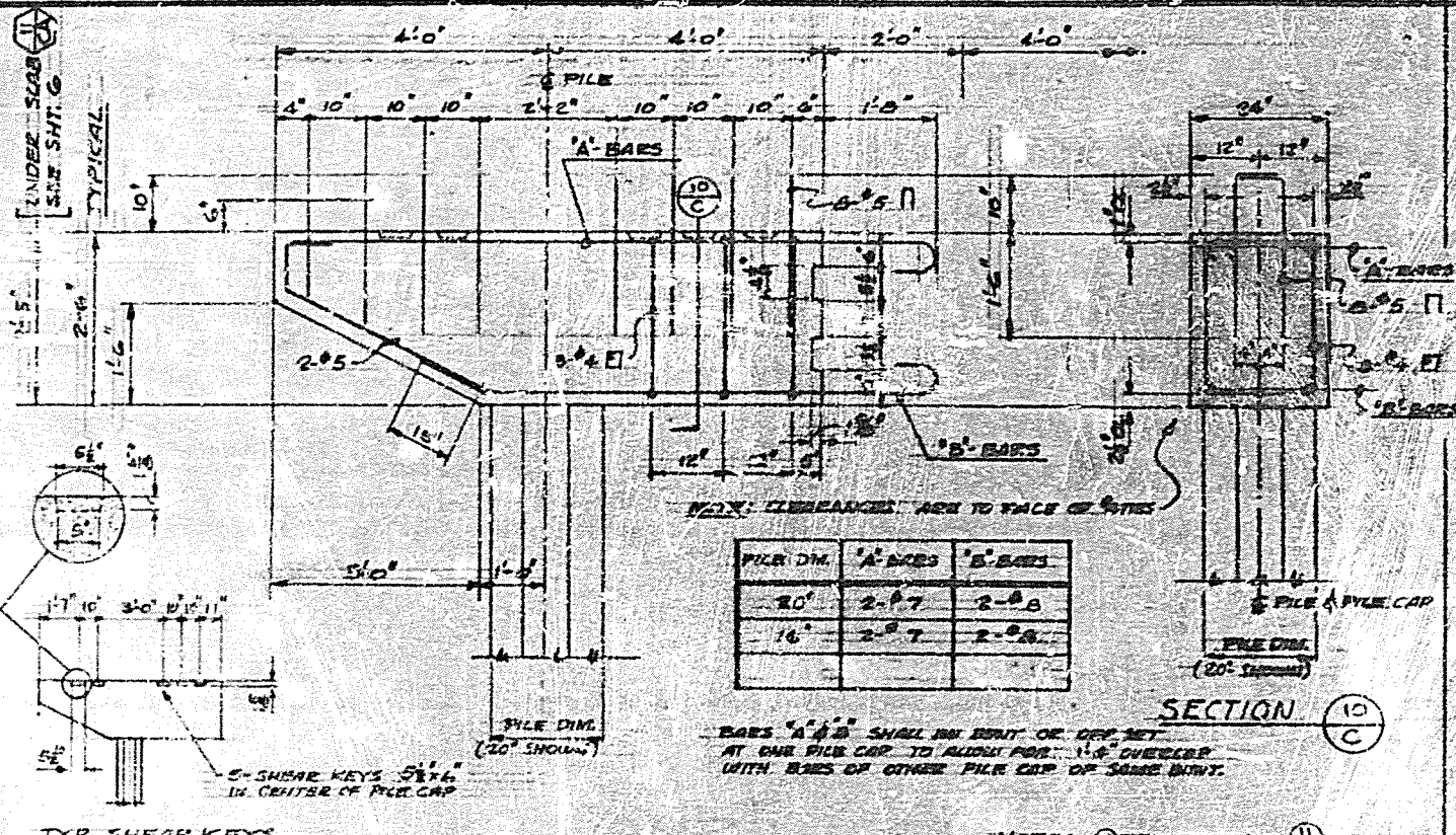
10 A TYP. PILE CAP DETAIL SCALE: 1/4" = 1'-0"
