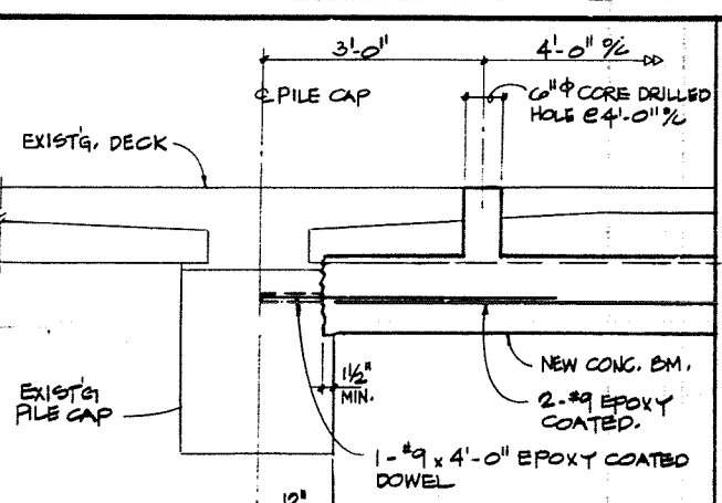
A3 CONN. OF NEW BM. TO EXIST. PILE CAPS
