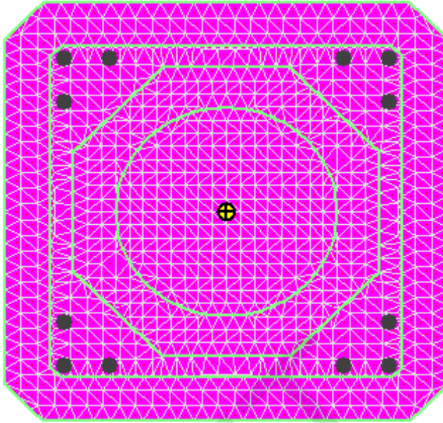
Figure 20 - Pile Jacket
