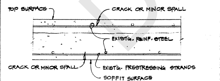
(B) 55 REPAIR FOR SPALLS & DELAMINATED AREAS IN SOFFIT OF DECK
