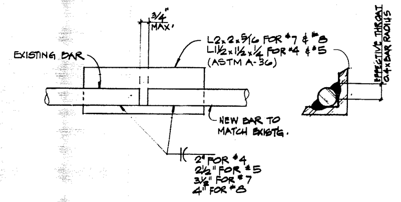
INDIRECT BUTT SPLICE
