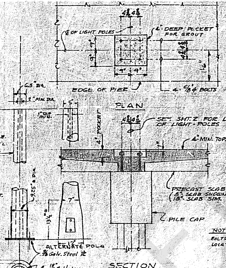
LIGHT-POLE BASE DETAIL SCALE: 3/4" = 1'-0"
