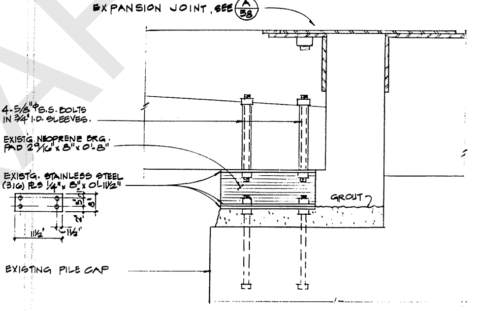
D 56 DETAIL OF EXISTING BEARING PADS AT EXPANSION JOINTS 3" = 1'-0"
