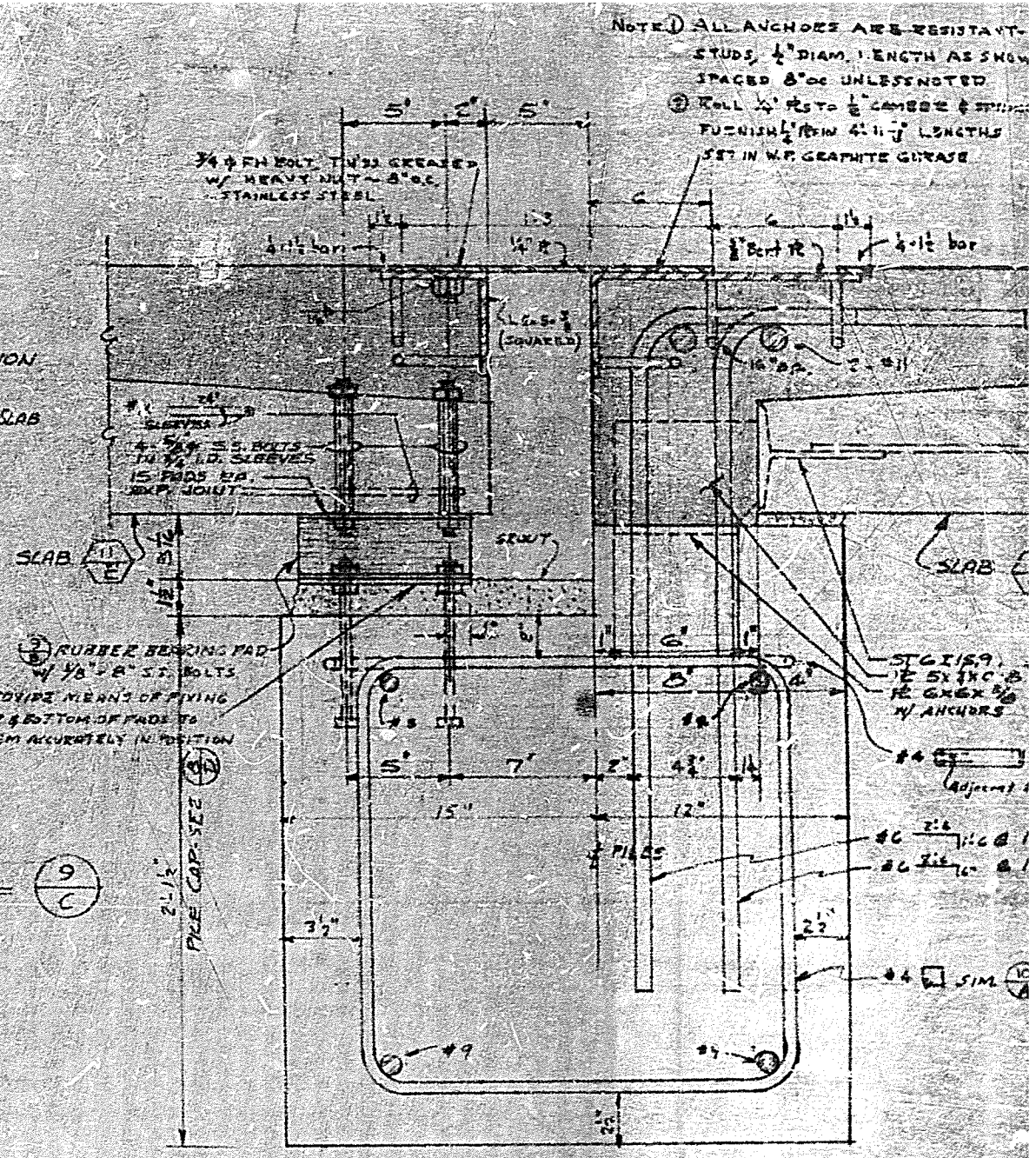
SECT. THRU PILE CAP @ EXPANSION JT. - TYP.
