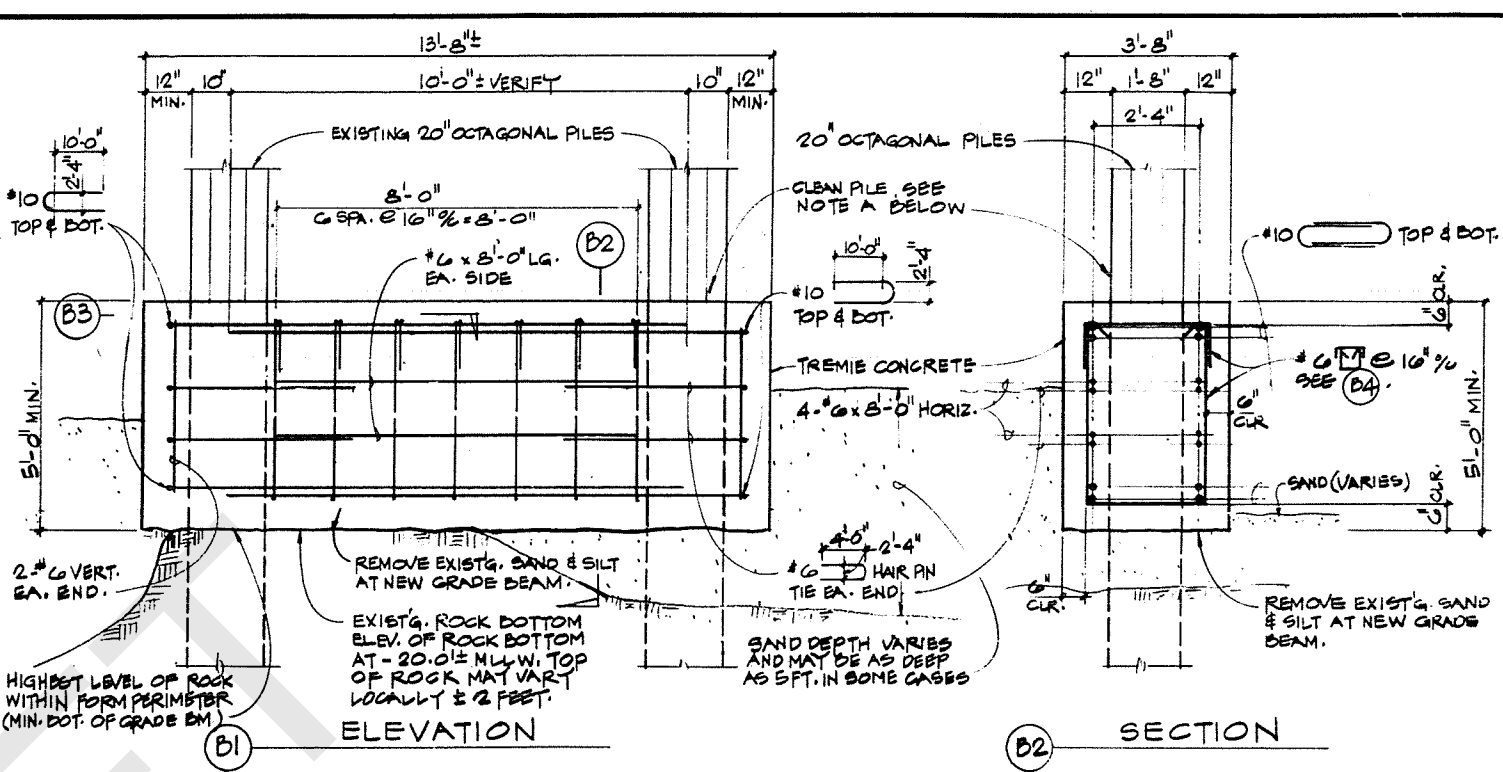
A3 CONN. OF NEW BM. TO EXIST. PILE CAPS
