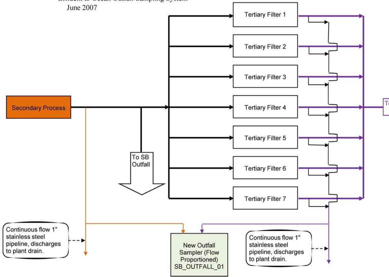
Figure 2 - Detail of Effluent Sampling System
