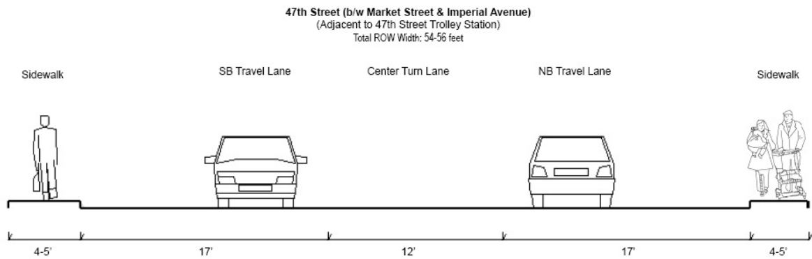
Figure 4-2L: Existing Right-of-way Dimensions: 47 th Street
