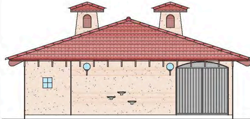
EAST ELEVATION - PROPOSED ORGAN PAVILION RESTROOM-OPTION 4B
