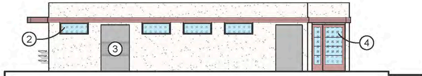
EAST ELEVATION - PROPOSED PALISADES RESTROOM
