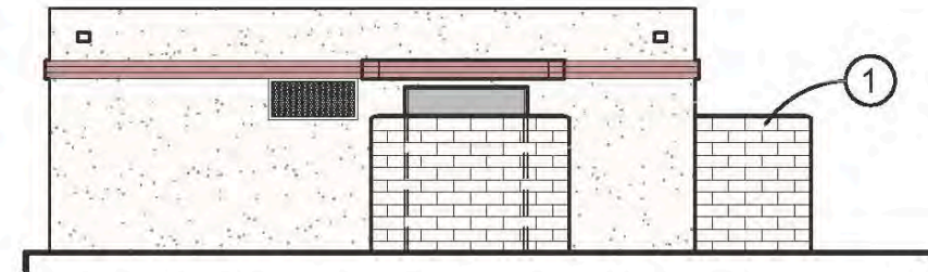
SOUTH ELEVATION - EXISTING
