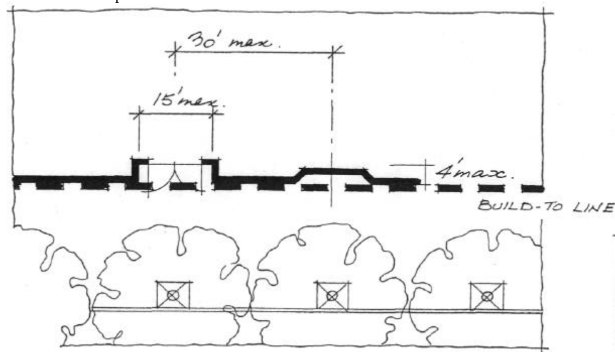
Build-to Line
