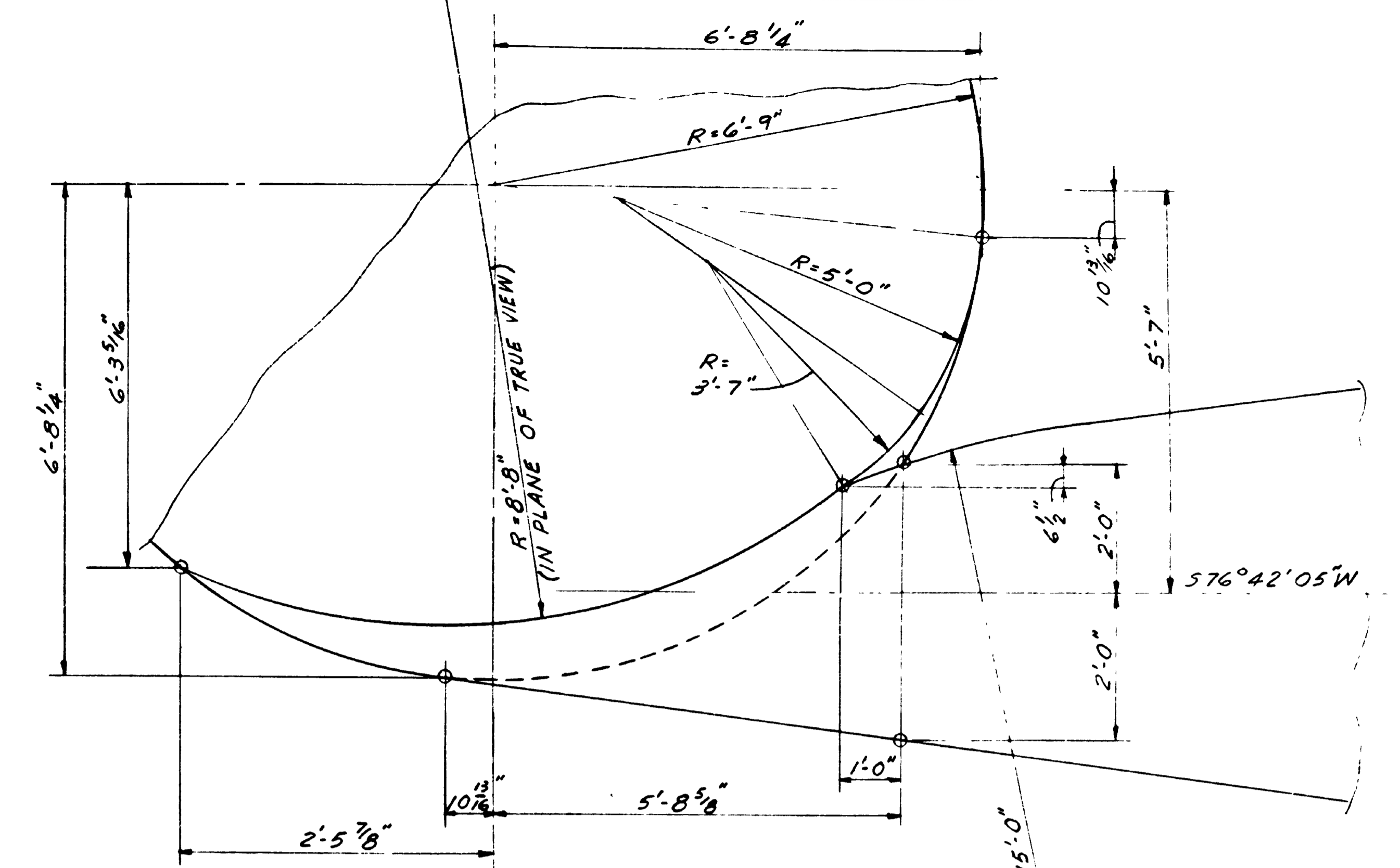
VORTEX SILL LAYOUT-DETAIL 1 NO SCALE
