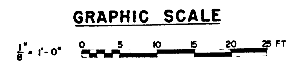
CONSTRUCTION SECTION F SCALE: 1/8" = 1'-0"
