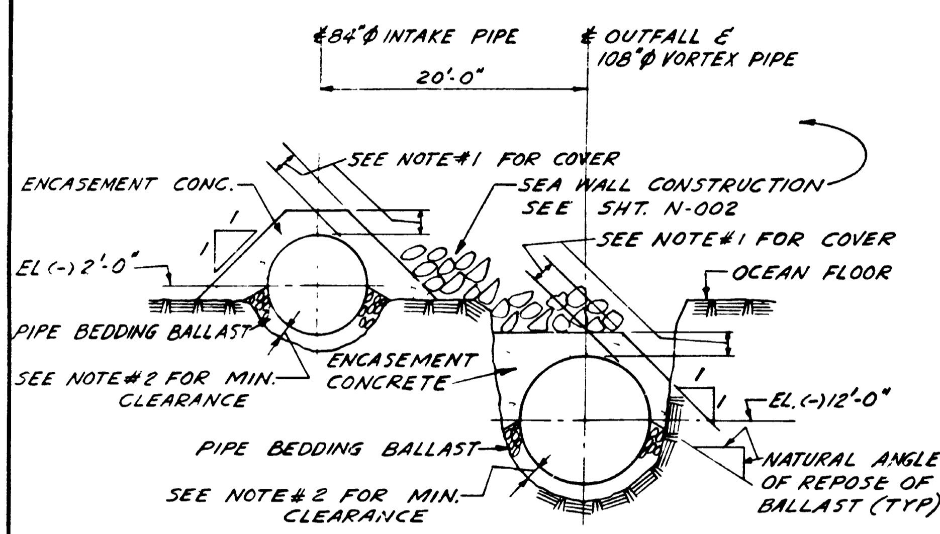
CONSTRUCTION SECTION E SCALE: 1/8" = 1'-0"
