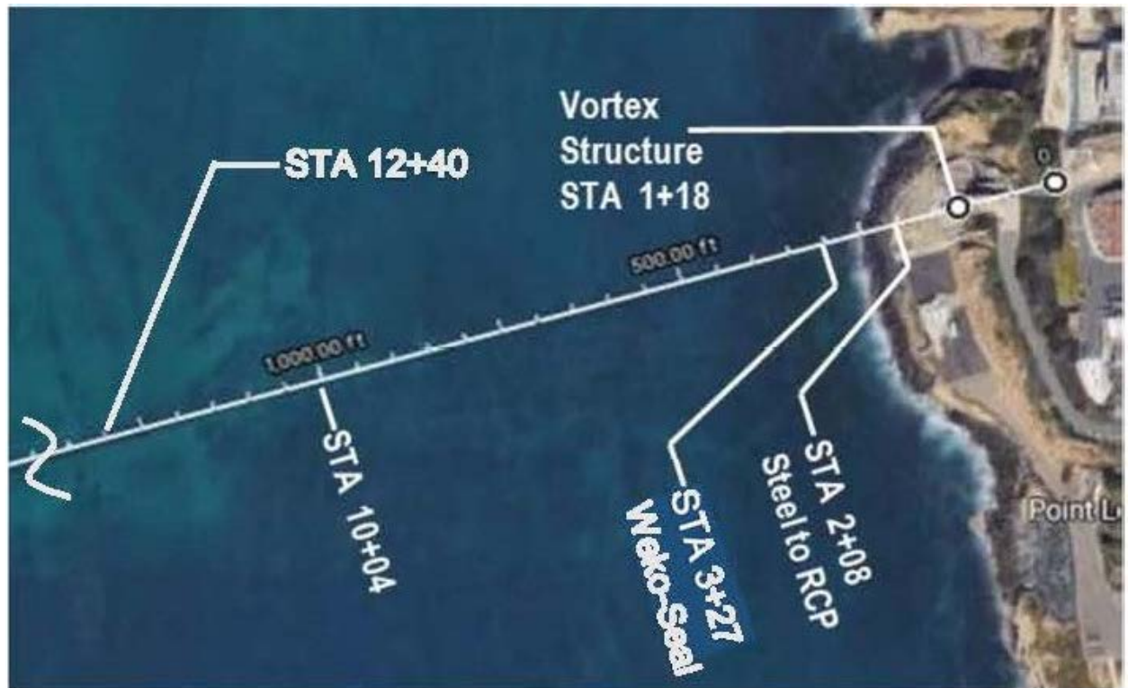
Outfall Stationing
