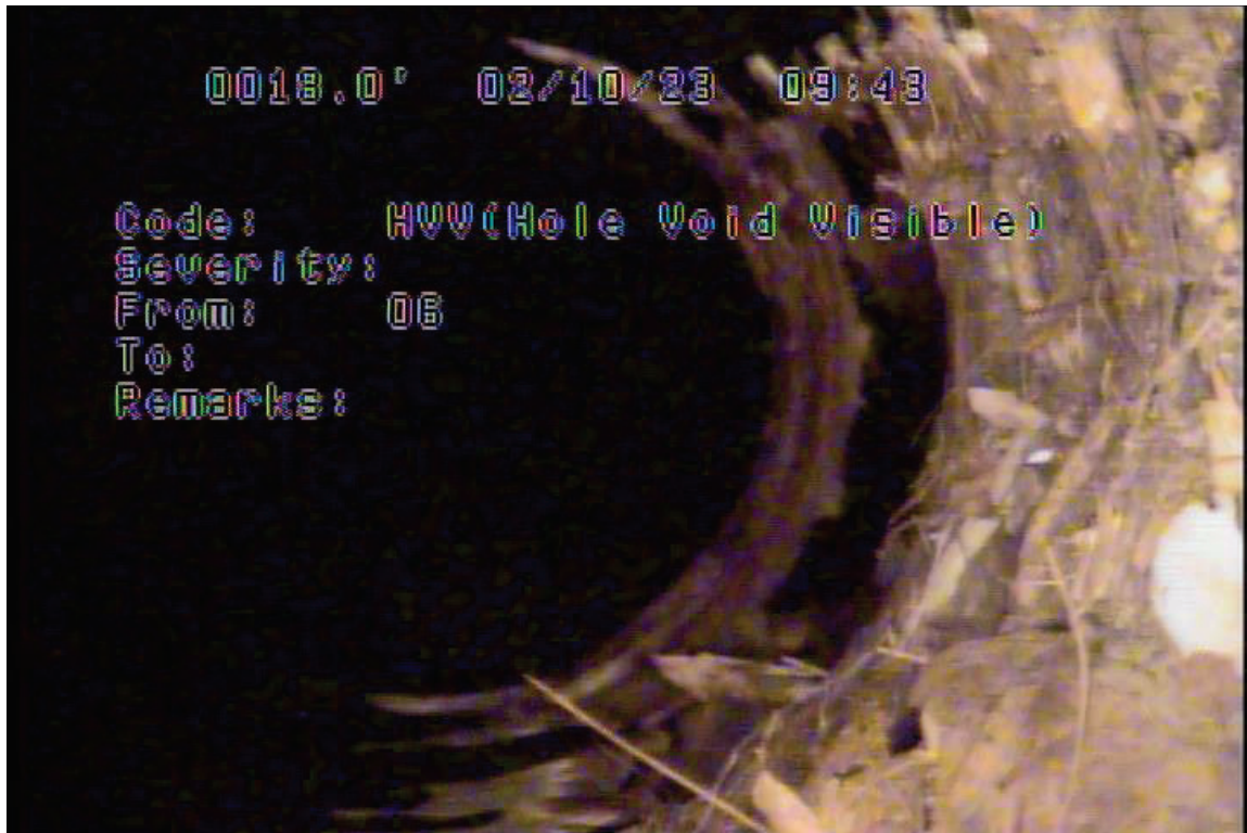
Figure 5 - Void present in CMP (2/10/23)
