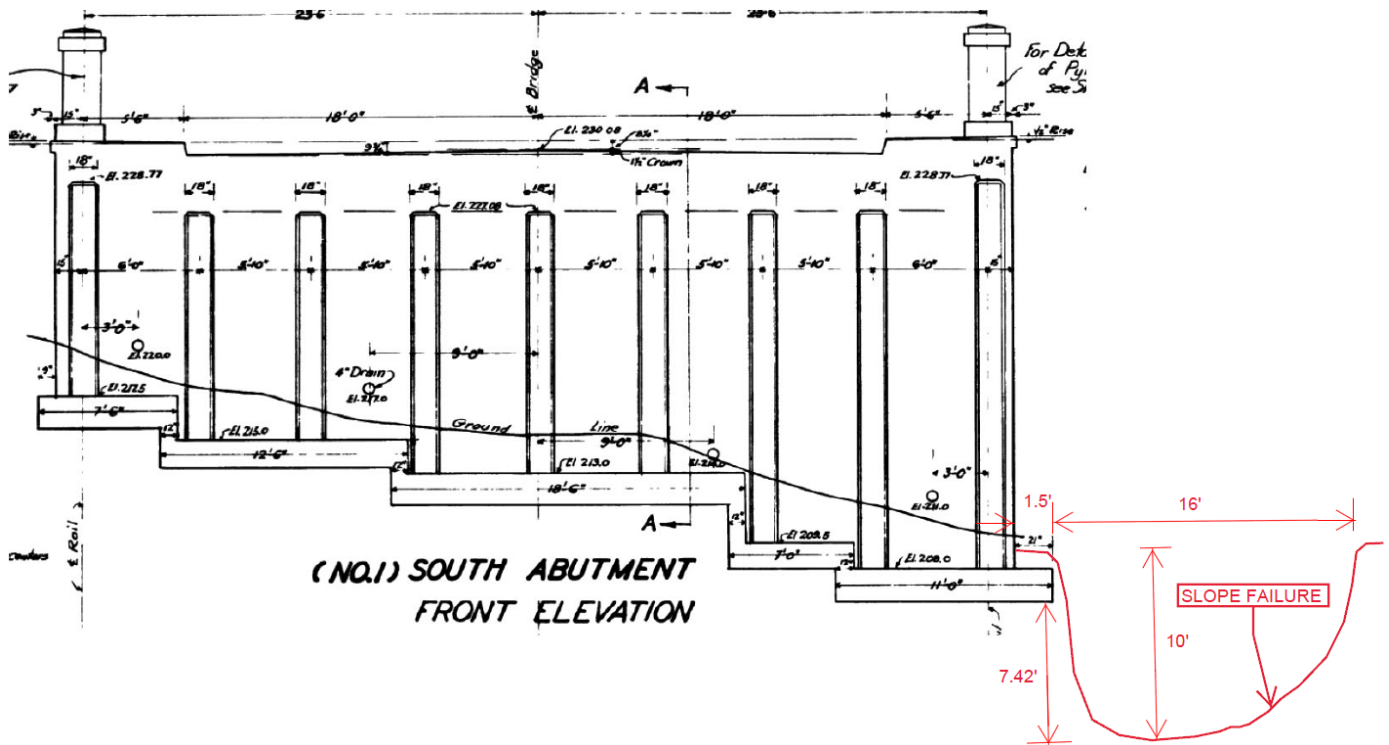
SOUTH ABUTMENT FRONT ELEVATION
