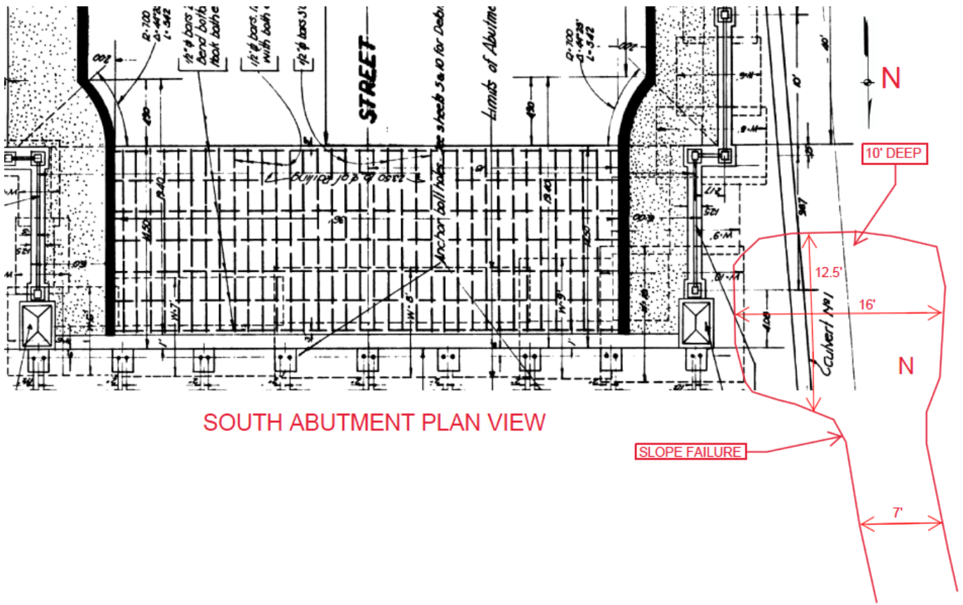
SOUTH ABUTMENT PLAN VIEW
