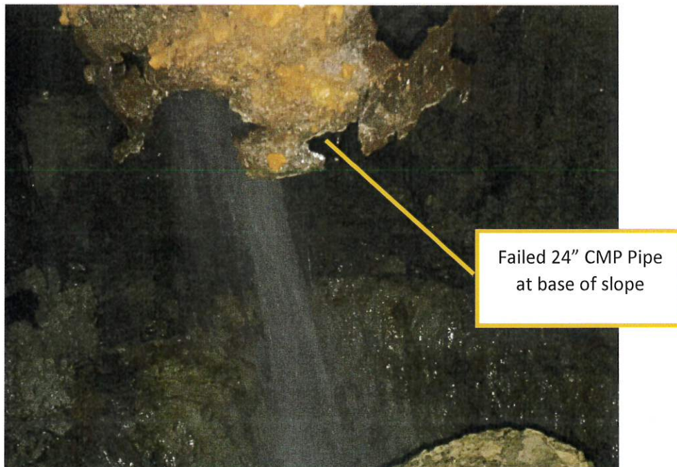
View of failed 24" CMP located within failed slope above 6 th Avenue
