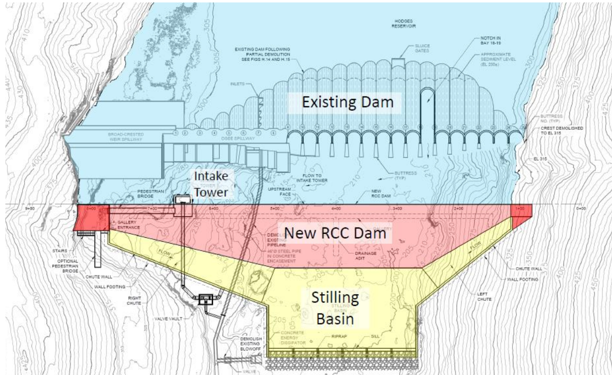
Lake Hodges Replacement Dam design drawing
