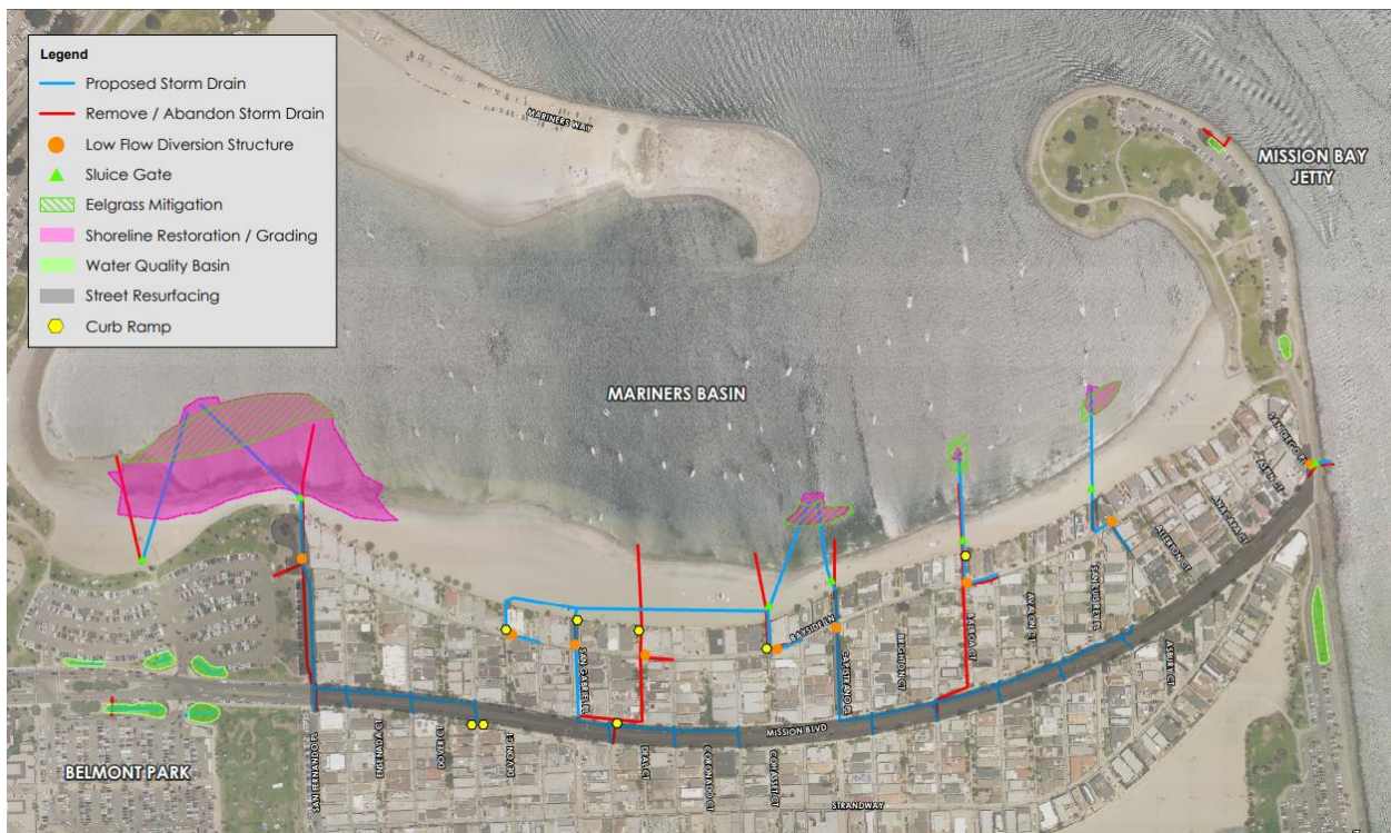
Proposed South Mission Beach Storm Drain project
